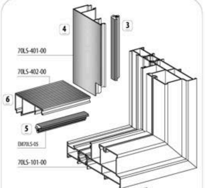
B C CORNER DETAIL / KÖŞE DETAYI
