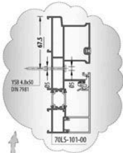
B DETAIL / DETAYI
