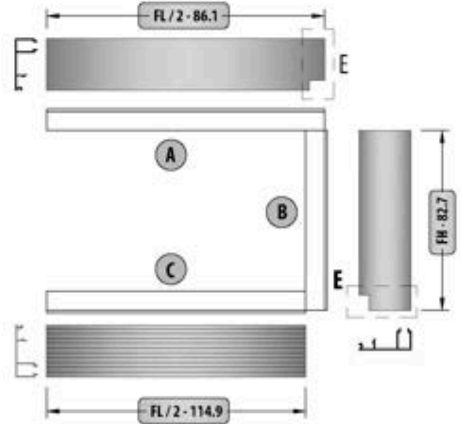
B C CORNER DETAIL / KÖŞE DETAYI
